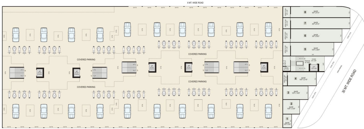
GROUND FLOOR PLAN - PARKING
